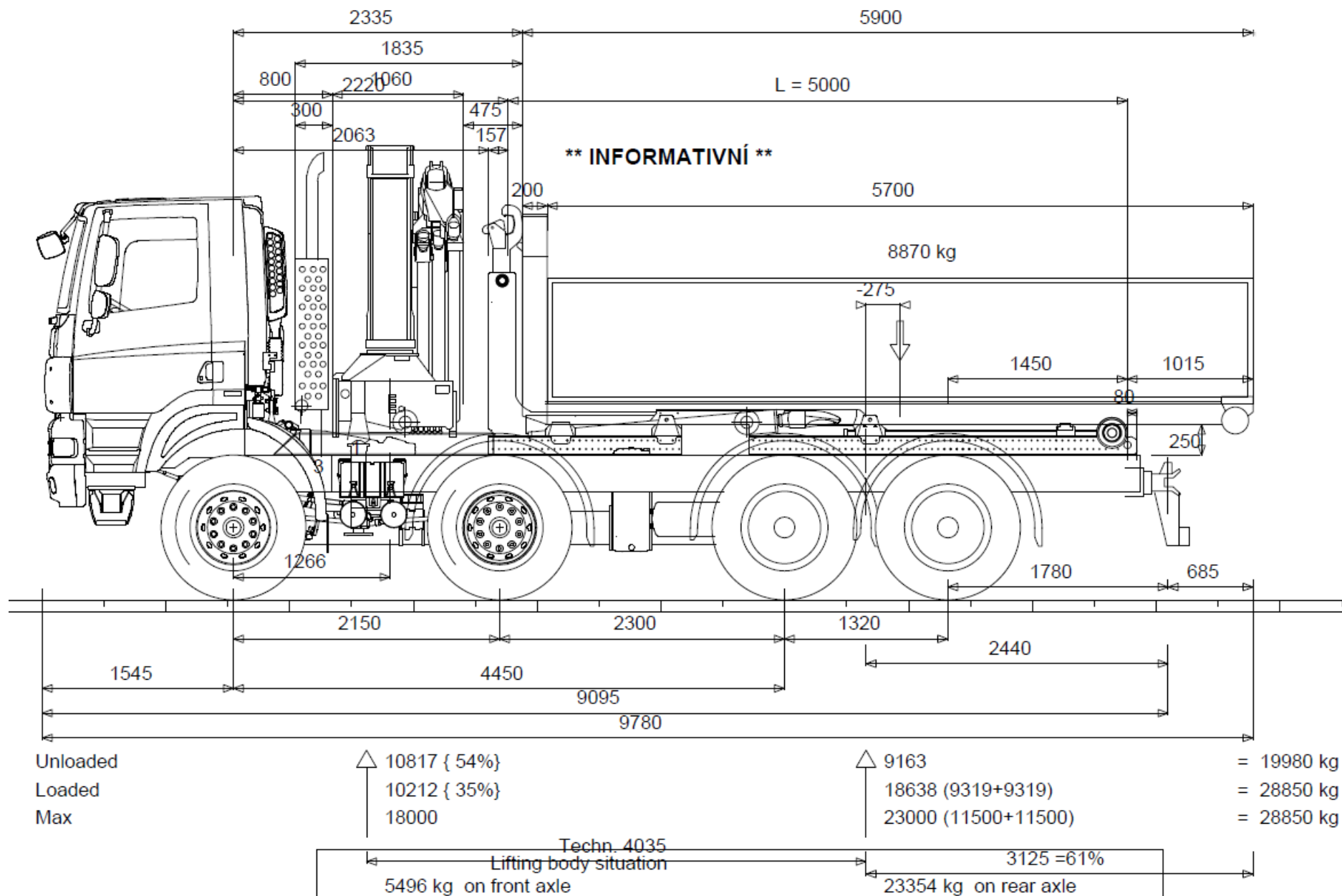
Tatra Phoenix Euro6 s hydraulickou rukou HMF 2820 – K6
